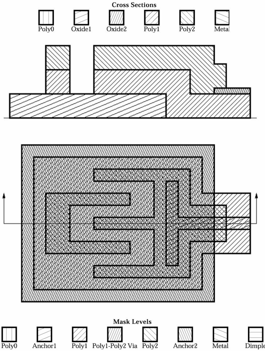
FIGURE 2.21. Design of double thickness structures. The upper figure shows the cross section of the structure after the Poly 2 has been deposited and etched (but before release).
