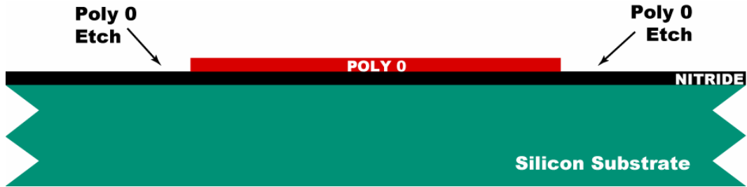
FIGURE 1.4. Plasma etching is used to remove the unwanted polysilicon. After the etch, the photoresist is chemically stripped in a solvent bath. This method of patterning the wafers with photoresist, etching and stripping the remaining photoresist is used repeatedly in the PolyMUMPs process.
