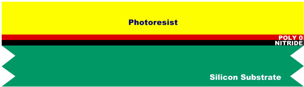
FIGURE 1.2. The surface of the starting n-type (100) wafers are heavily doped with phosphorus in a standard diffusion furnace using a PSG film as the dopant source. After removal of this PSG film, a 600 nm blanket layer of low stress silicon nitride (Nitride) is deposited followed by a blanket layer of 500 nm polysilicon (Poly 0). The wafers are then coated with UV-sensitive photoresist.
