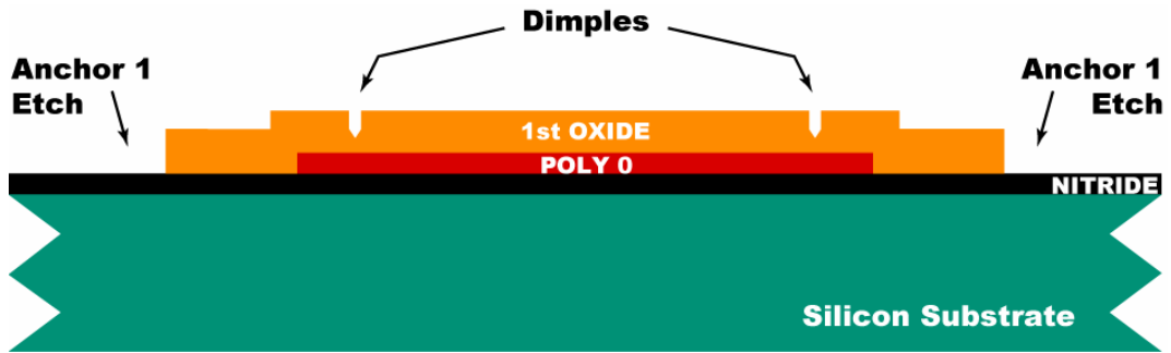
FIGURE 1.7. The wafers are re-coated with photoresist and the third level (ANCHOR1) is lithographically patterned. The unwanted oxide is removed in a RIE process and the photoresist is stripped.
